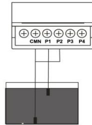
Draining Control (Single level Monitoring with two Sensors)
