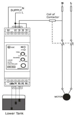
Draining Control (Single Tank Monitoring with 3 Sensors)
