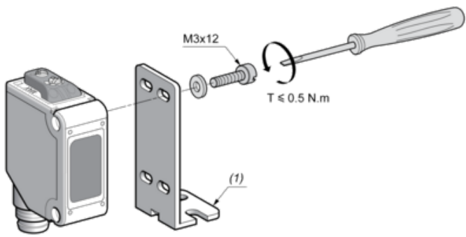
(1) Metal bracket
